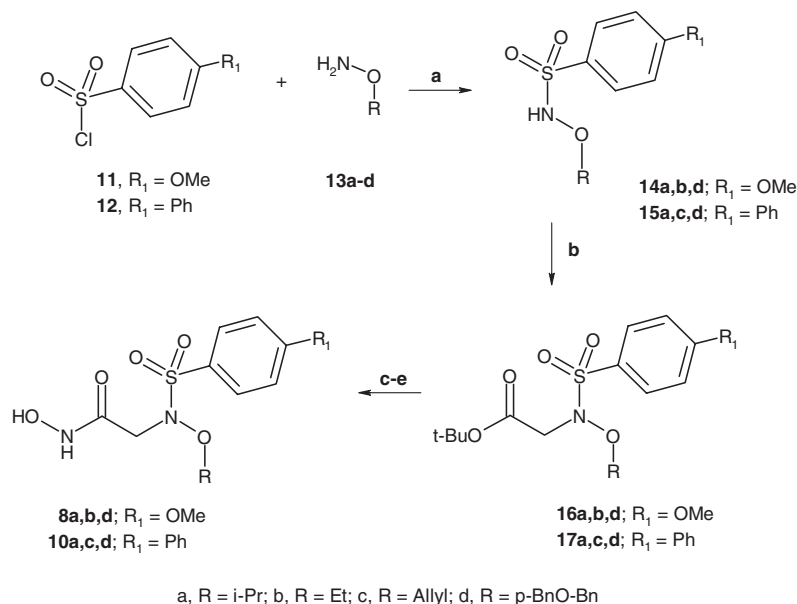
Scheme 1. Reagents and conditions: (a) NMM, anhyd THF, rt; (b) BrCH 2 CO 2 -Bu t , Cs 2 CO 3 , Bu 4 NHSO 4 , anhyd DMF, rt, 3 days; (c) TFA, anhyd CH 2 Cl 2 , 0 °C, 5 h; (d) TBDMSONH 2 , EDCI, anhyd CH 2 Cl 2 , 0–25 °C, 24 h; (e) TFA, anhyd CH 2 Cl 2 , 0 °C, 5 h.
